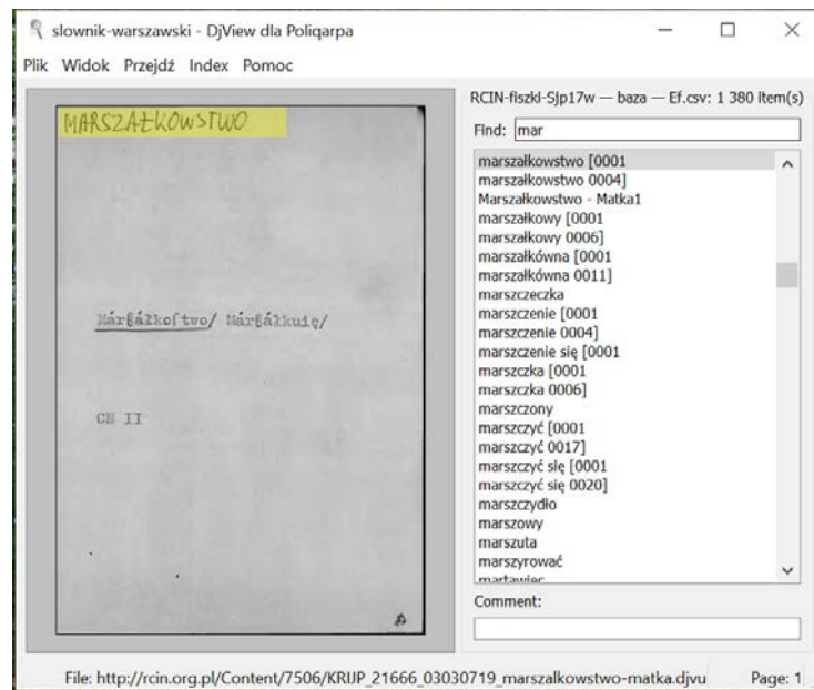
Figure 1. A screenshot of the djview4poliqarp software, scanned paper quotation slip marszałkostwo (English marshalcy ) and the test card index
